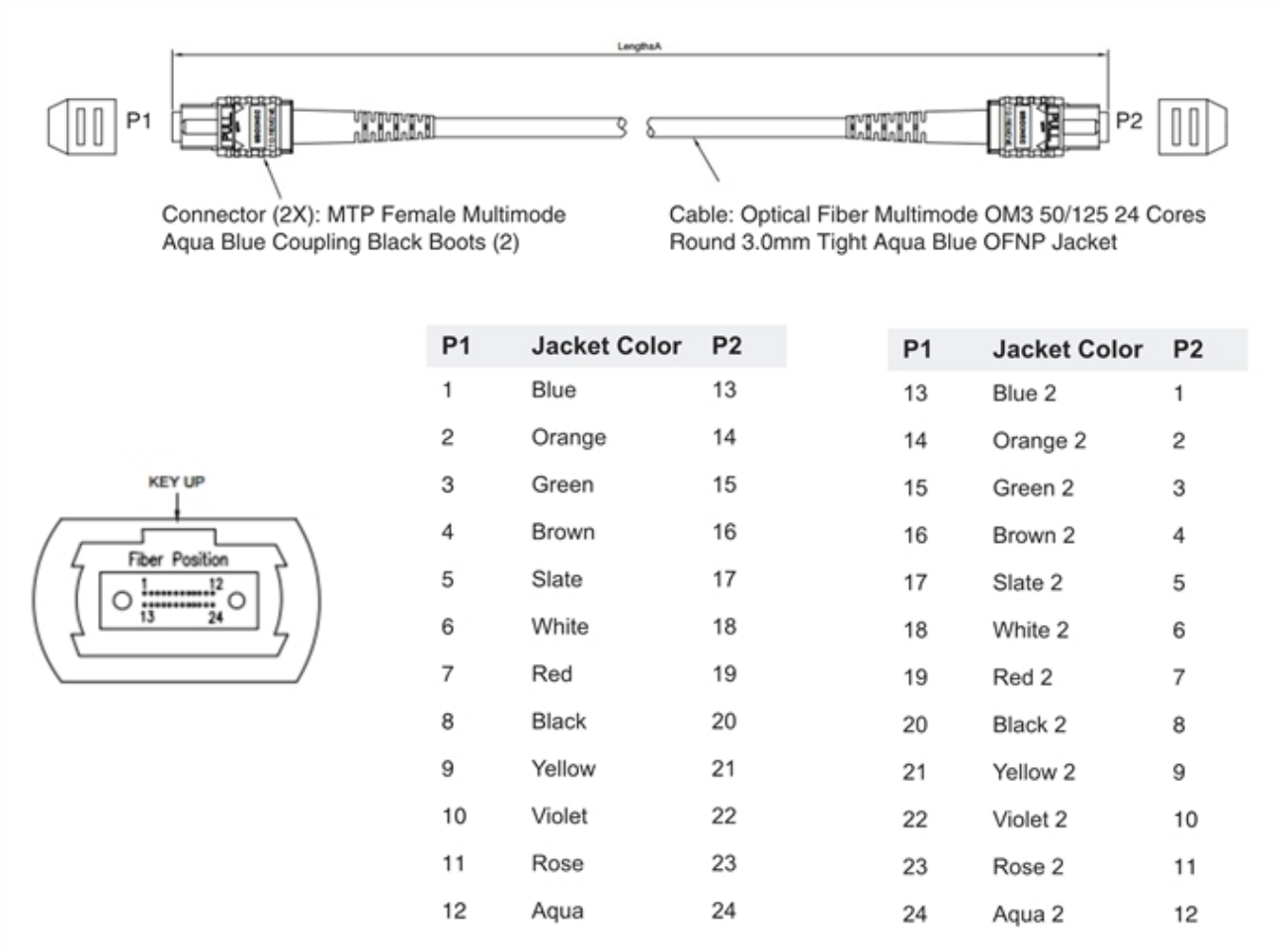
Figure 22 MPO/MTP 24 Position Fiber Cable
